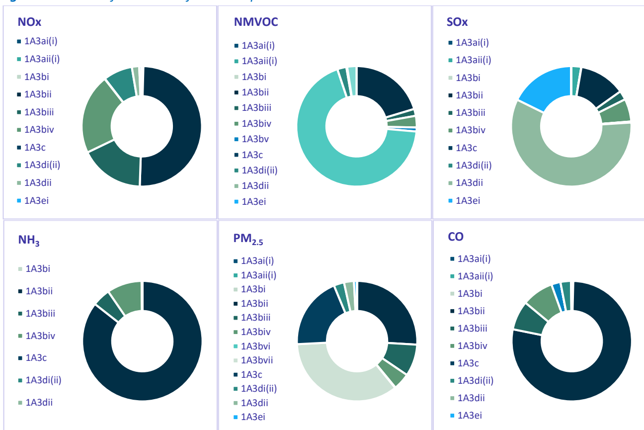
Figure 3.4: Share of emissions of the main pollutants in 1A3 in 2022
