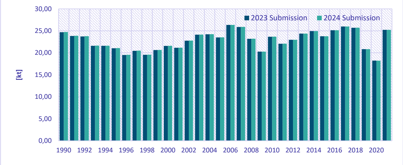
Figure 8.14: Comparison of PCBs emission total between the 2023 final submission and 2024 final submission
