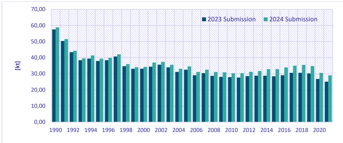
Figure 8.4: Comparison of NH 3 emission total between the 2023 final submission and 2024 final submission
