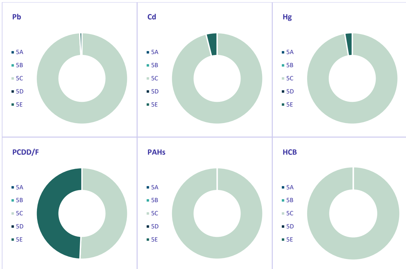
Figure 6.4: Share of subsectors of the waste sector on emissions of the HMs and POPs in 2022
