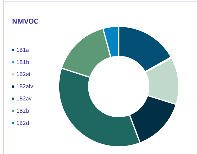
Figure 3.10: Share of emissions of NMVOC in 1B in 2022
