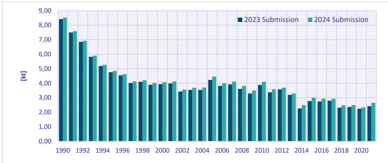
Figure 8.6: Comparison of BC emission total between the 2023 final submission and 2024 final submission
