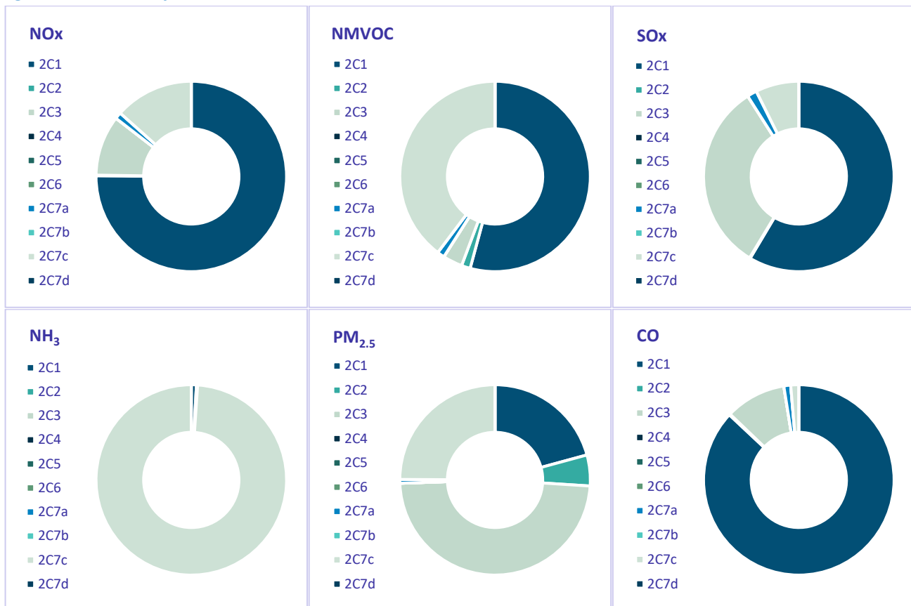
Figure 4.5: Shares of emissions in 2C in 2022
