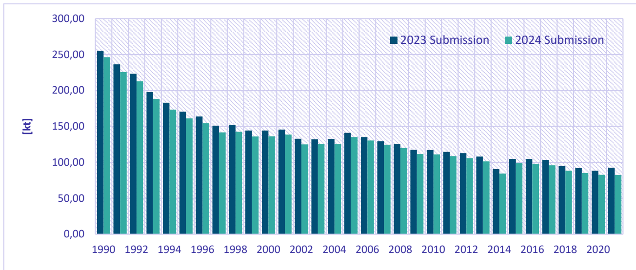
Figure 8.2: Comparison of NMVOC emission total between the 2023 final submission and 2024 final submission
