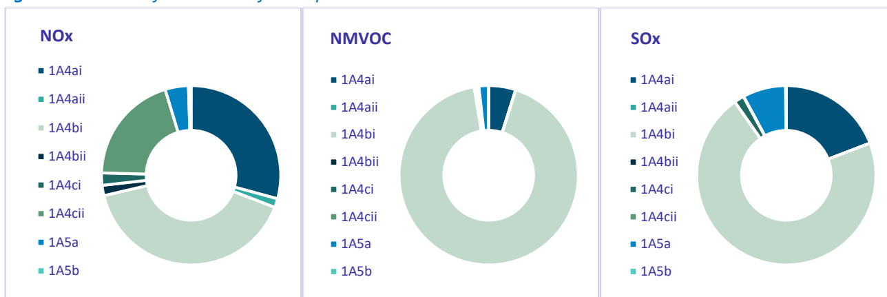
Figure 3.9: Share of emissions of main pollutants in 1A4 and 1A5 in 2022
