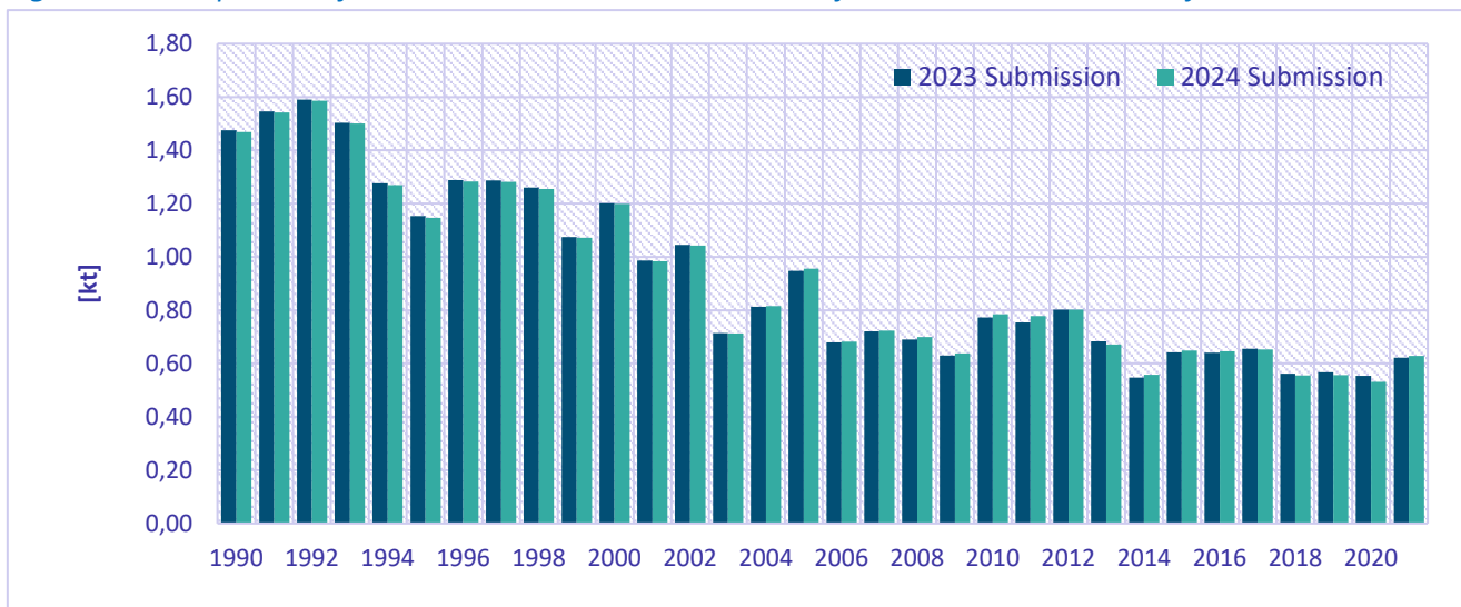
Figure 8.10: Comparison of Hg emission total between the 2023 final submission and 2024 final submission
