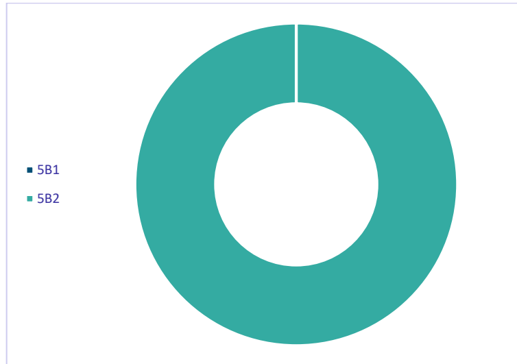
Figure 6.5: Share of NH 3 emissions of individual categories in 5B in 2022
