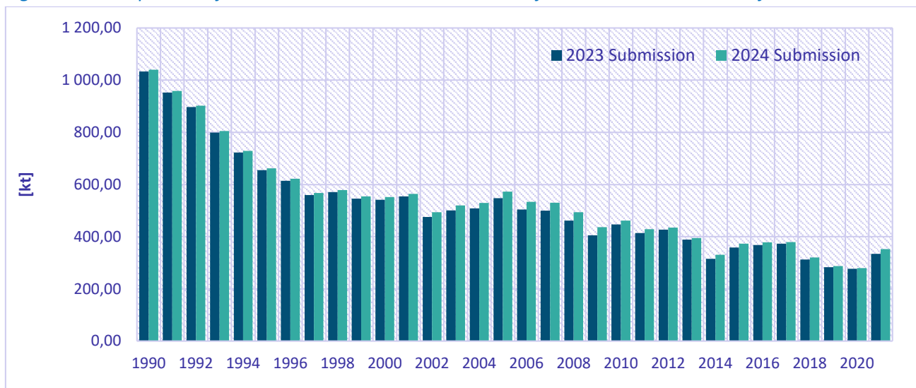
Figure 8.7: Comparison of CO emission total between the 2023 final submission and 2024 final submission
