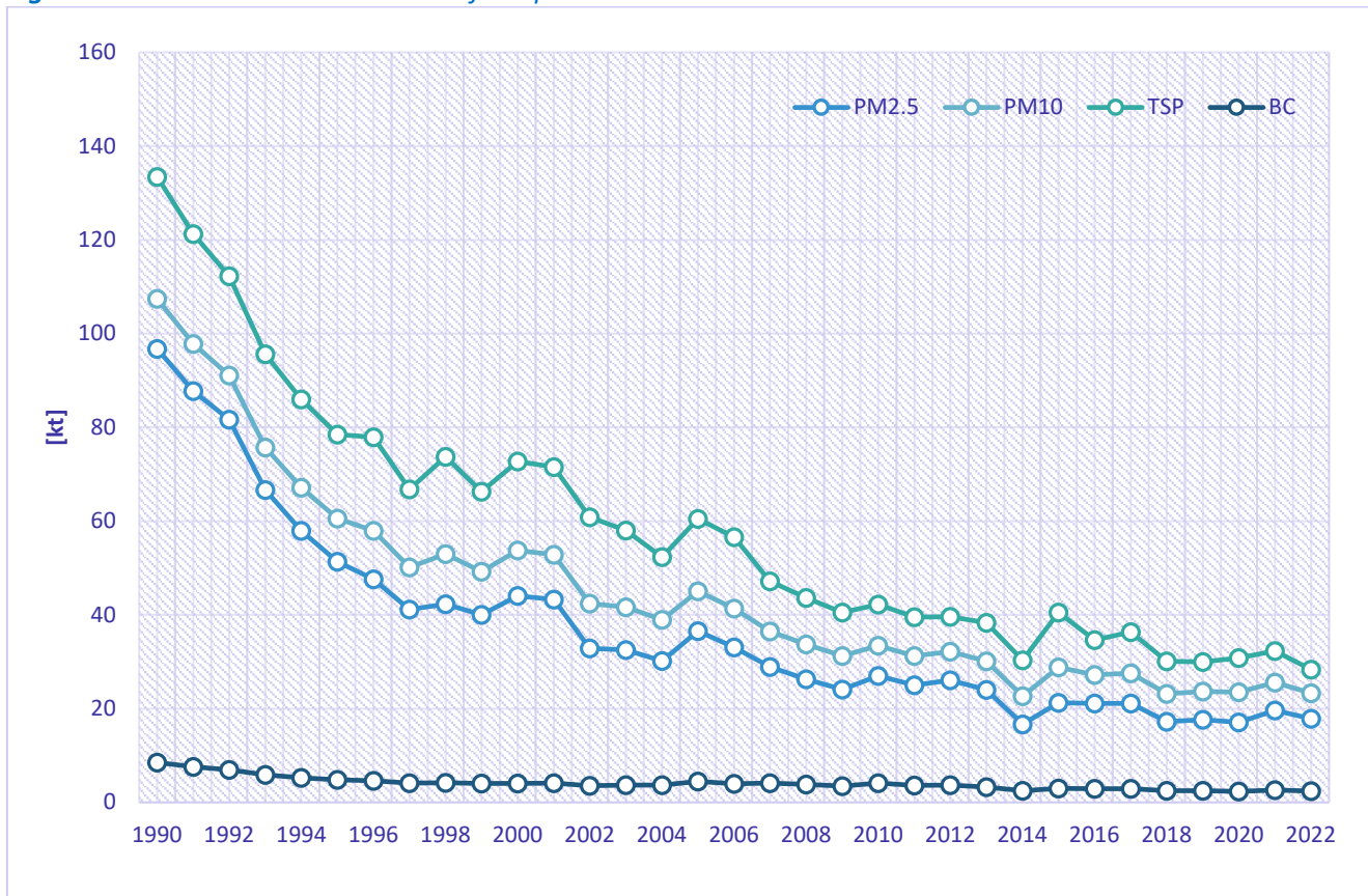
Figure ES.2: Overall emission trends of the particulate matter
