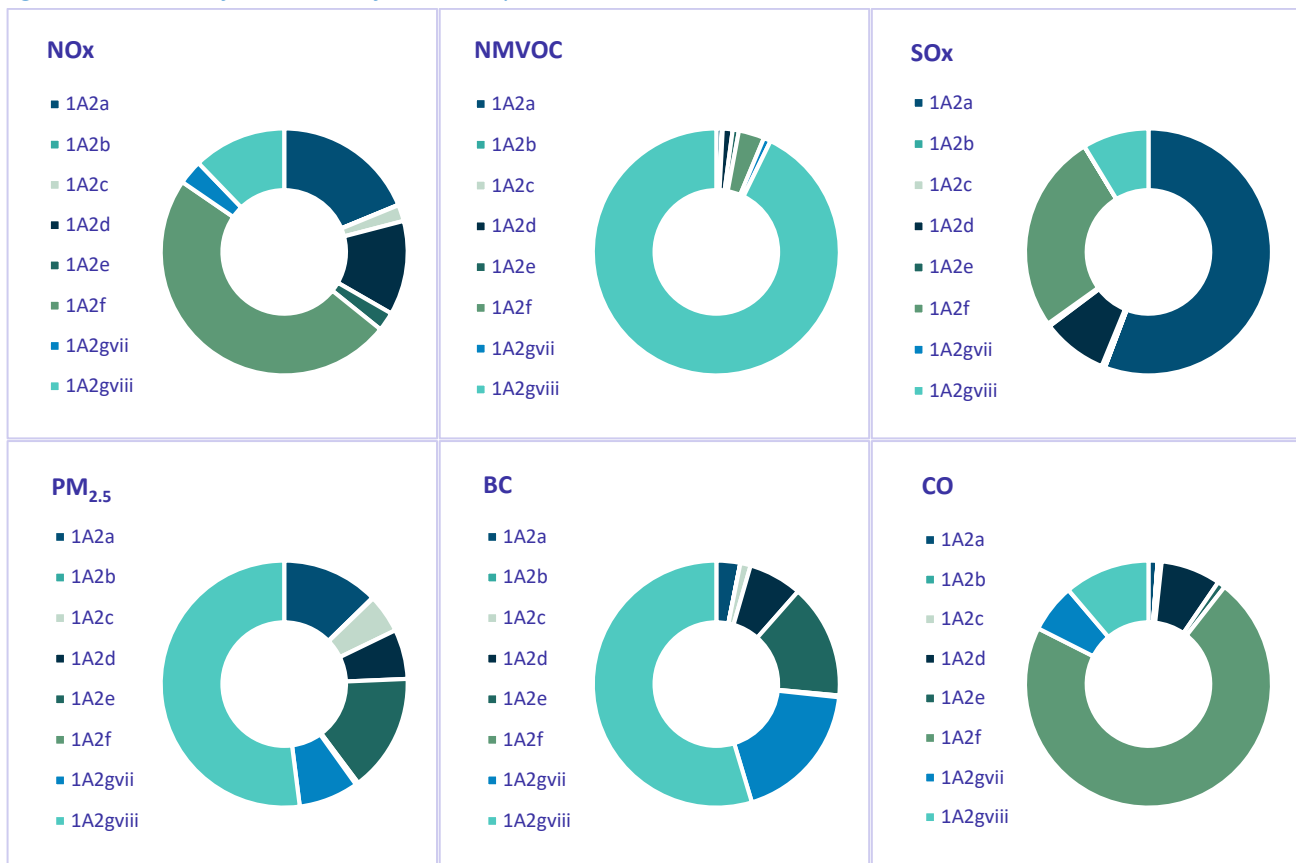
Figure 3.3: Share of emissions of the main pollutants in 1A2 in 2022
