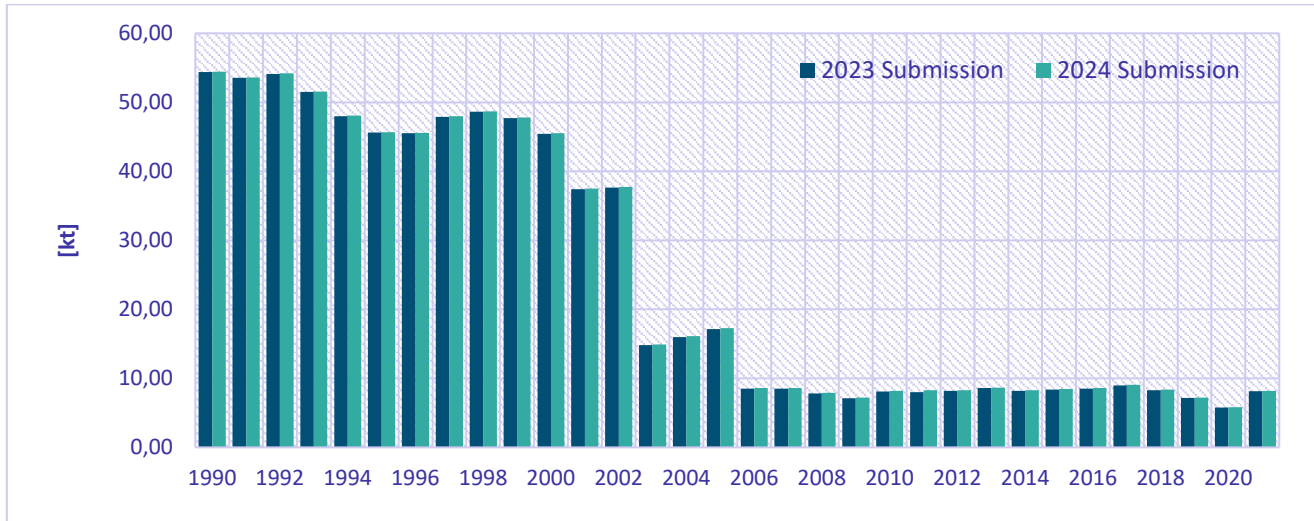
Figure 8.9: Comparison of Cd emission total between the 2023 final submission and 2024 final submission
