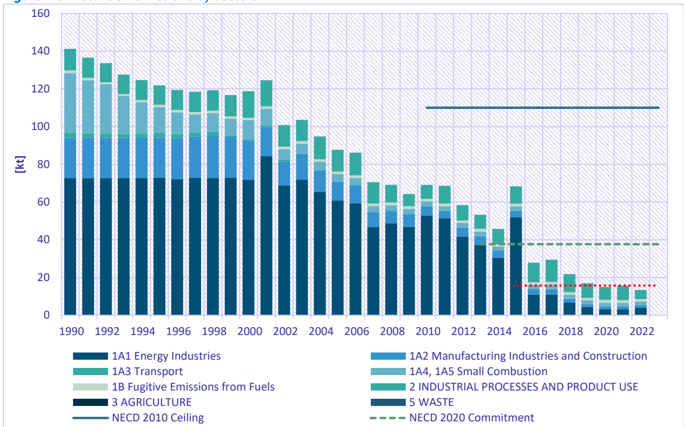
Figure 2.3: Total SOx emissions by sectors
