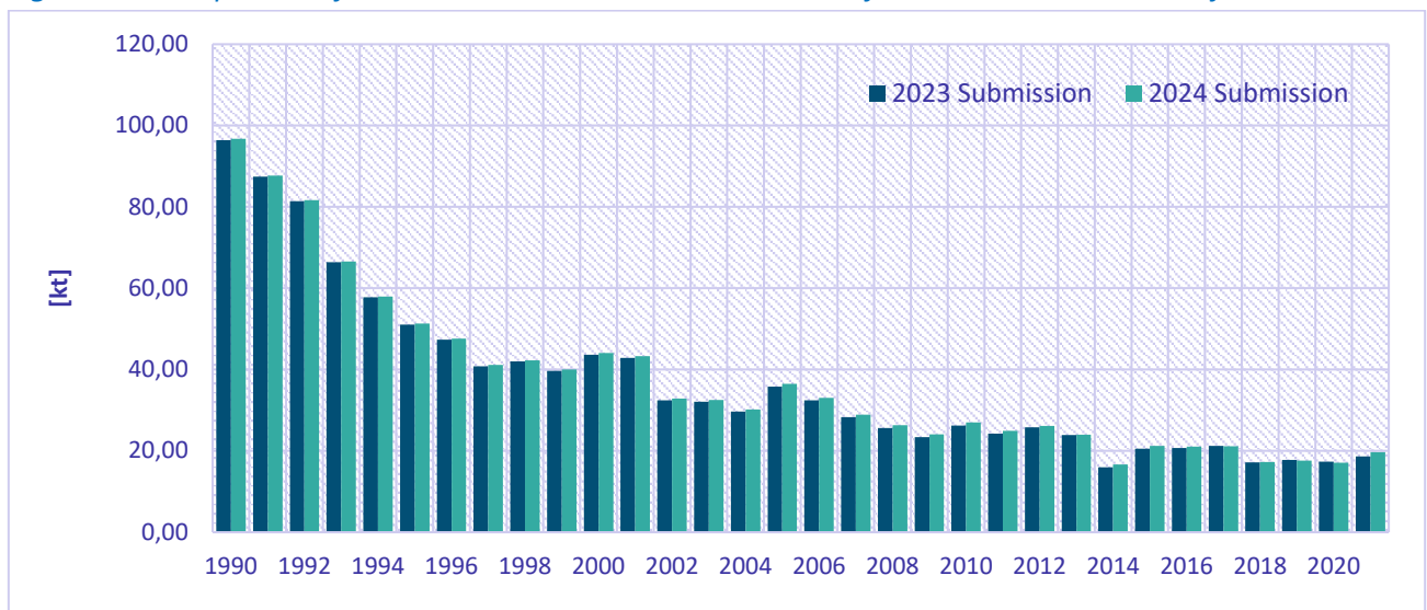
Figure 8.5: Comparison of PM 2.5 emission total between the 2023 final submission and 2024 final submission
