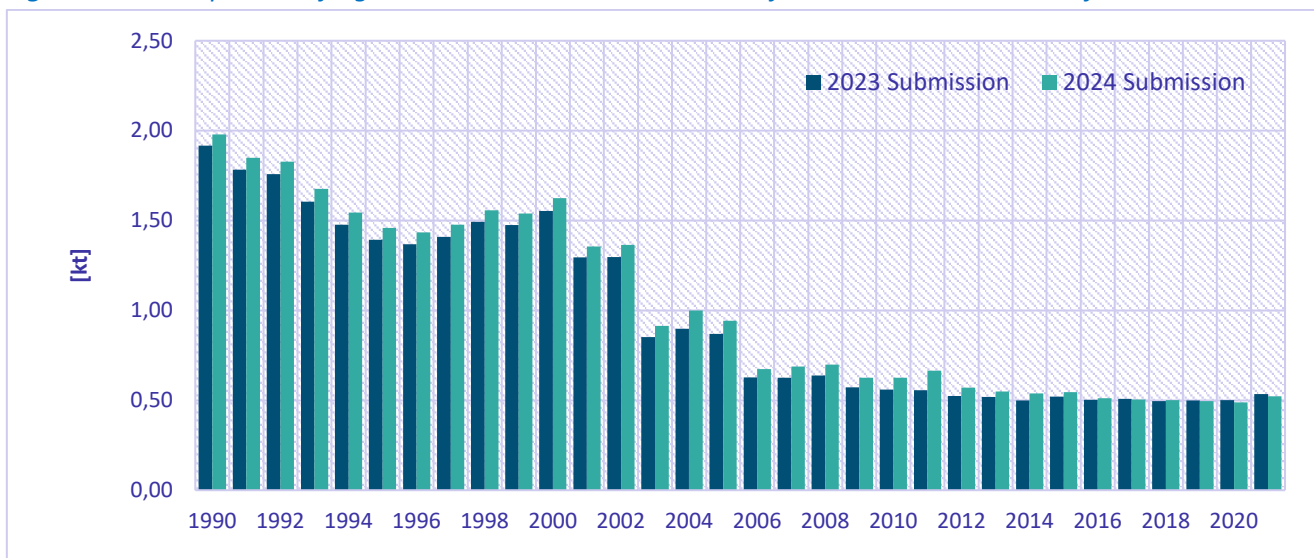
Figure 8.10: Comparison of Hg emission total between the 2023 final submission and 2024 final submission
