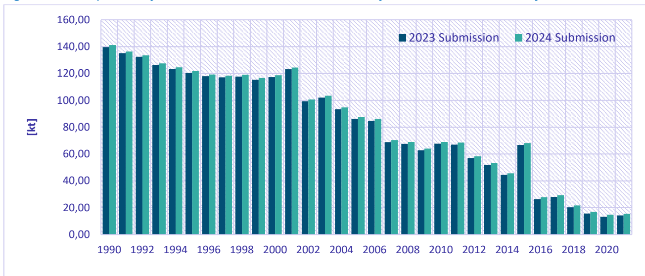
Figure 8.3: Comparison of SOx emission total between the 2023 final submission and 2024 final submission
