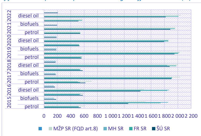
Figure 3.5: Results of fuels consumption comparison according to different sources (kt)
