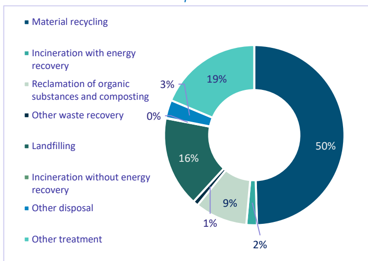
Figure 6.2: Industrial waste treatment in the Slovak Republic in 2022
