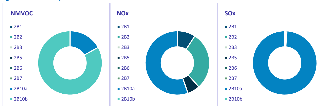
Figure 4.4: Shares of emissions in 2B in 2022
