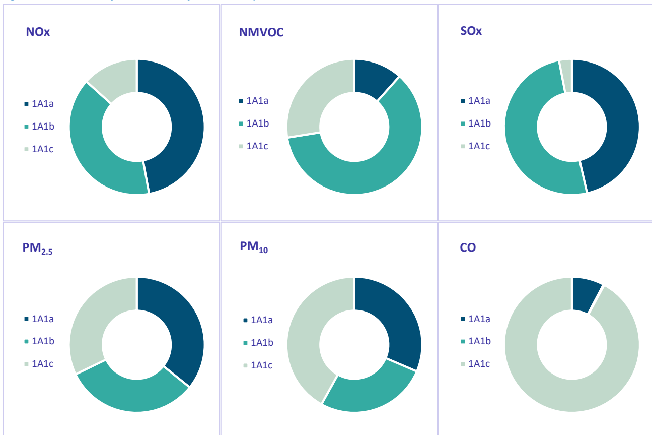
Figure 3.2: Share of emissions of the main pollutants in 1A1 in 2022
