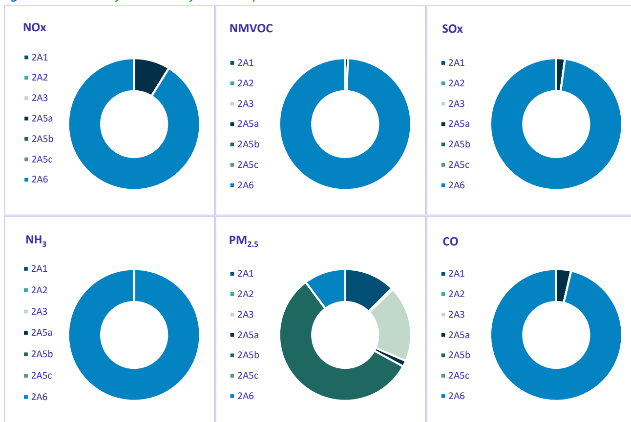
Figure 4.3: Shares of emissions of the main pollutants in 2A in 2022
