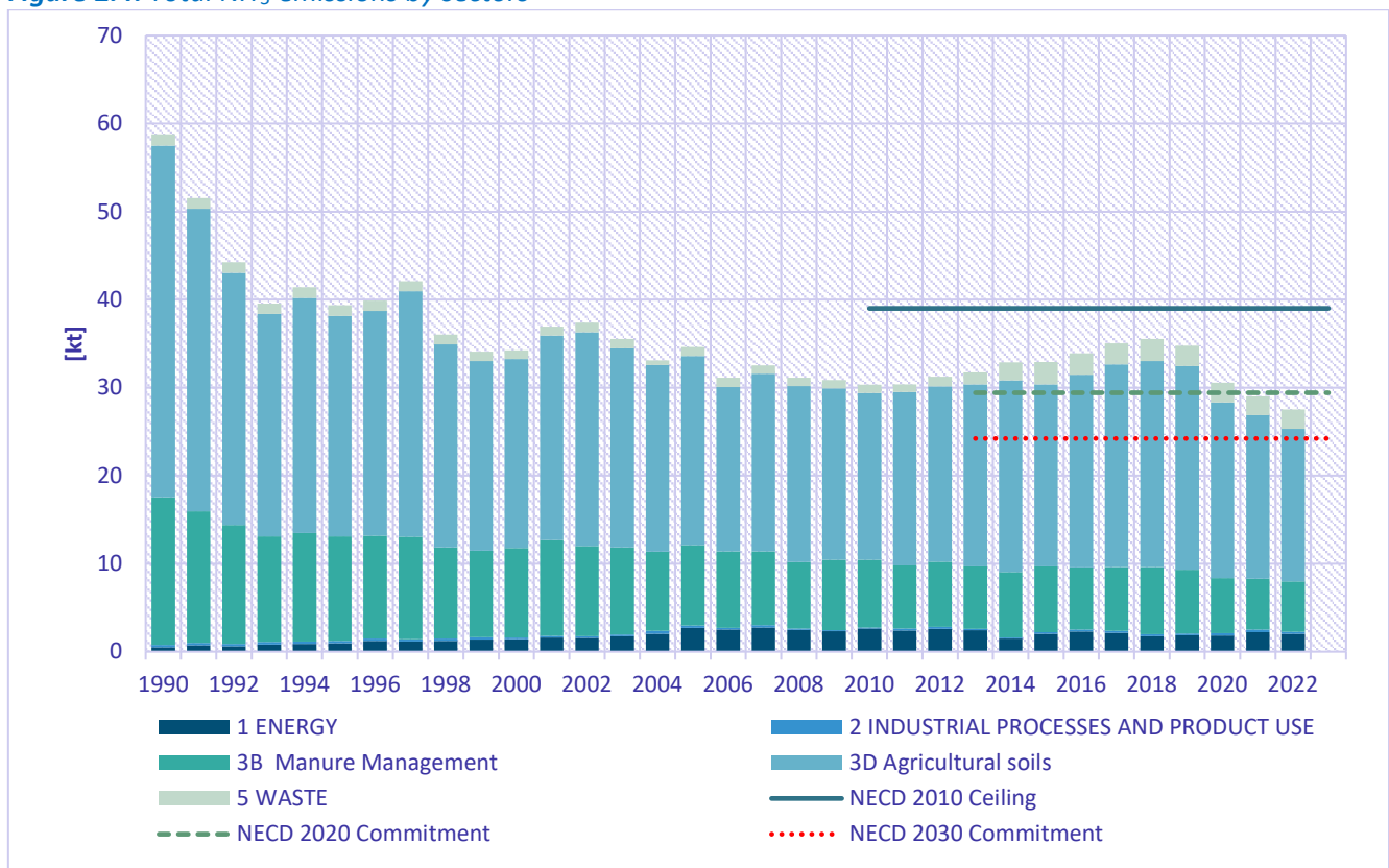
Figure 2.4: Total NH 3 emissions by sectors
