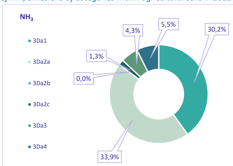
Figure 5.13: The share of NH 3 emissions by categories within agricultural soils in 2022
