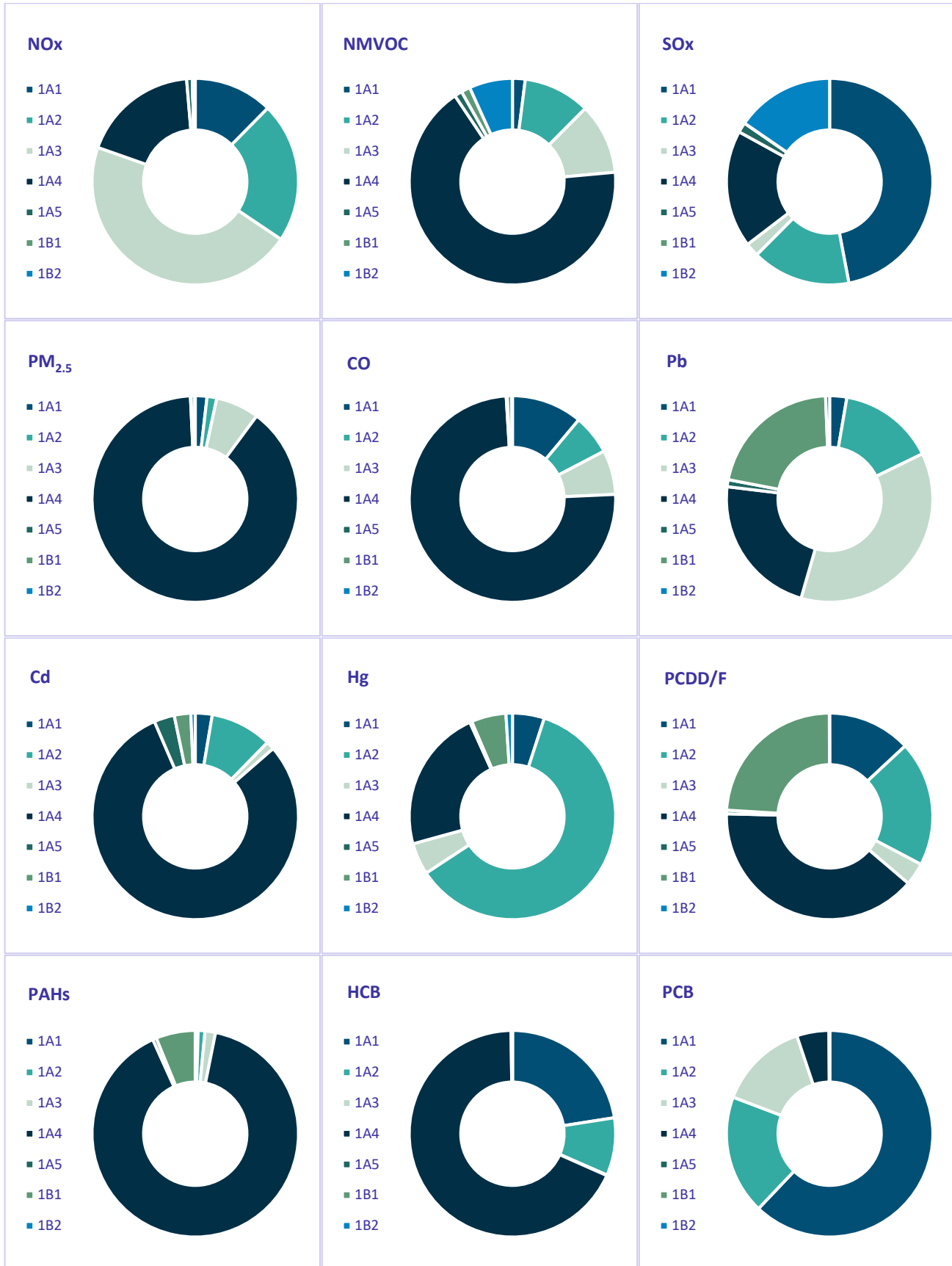
Figure 3.1: Share of the categories of emissions of the particular pollutants in the energy sector in 2022
