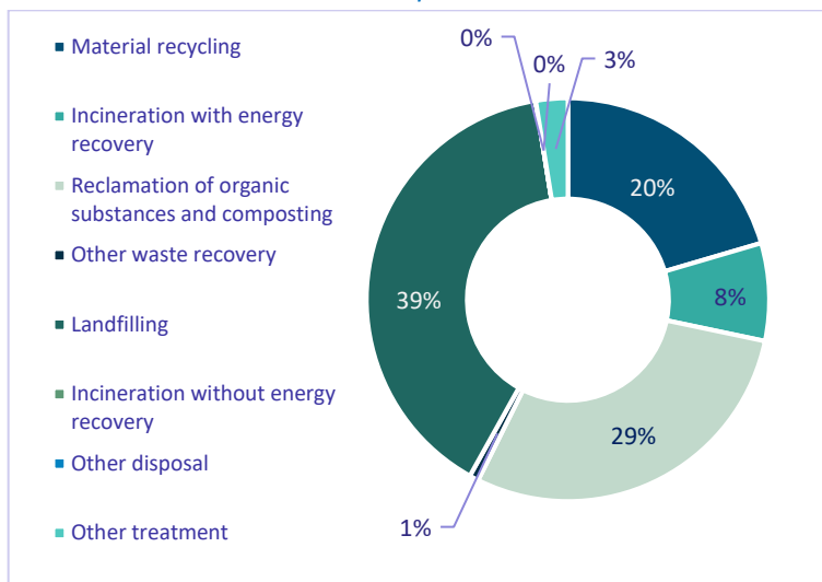
Figure 6.1: Municipal waste treatment in the Slovak Republic in 2022
