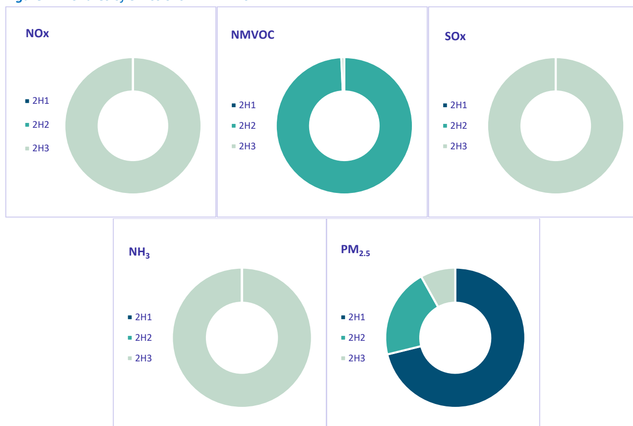
Figure 4.7: Shares of emissions in 2H in 2022
