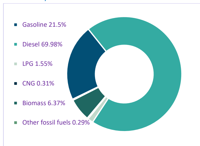
Figure 3.7: Fuels balance in road transportation in 2022
