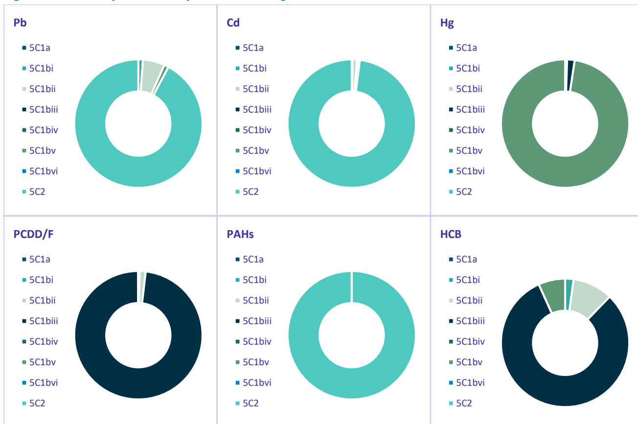
Figure 6.6: Share of emissions of individual categories in 5C in 2022
