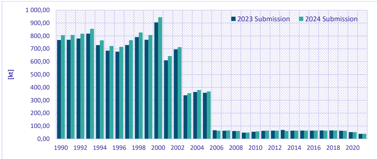
Figure 8.11: Comparison of PCDD/F emission total between the 2023 final submission and 2024 final submission
