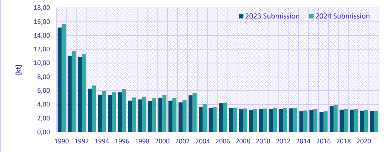
Figure 8.14: Comparison of PCBs emission total between the 2023 final submission and 2024 final submission
