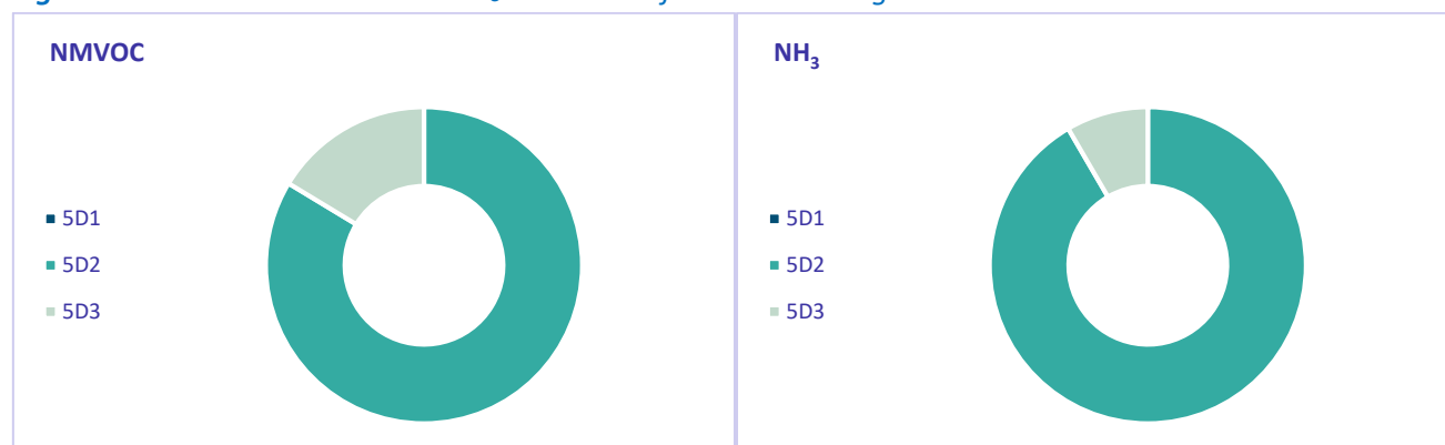
Figure 6.7: Share in NMVOC and NH 3 emissions of individual categories in 5D in 2022
