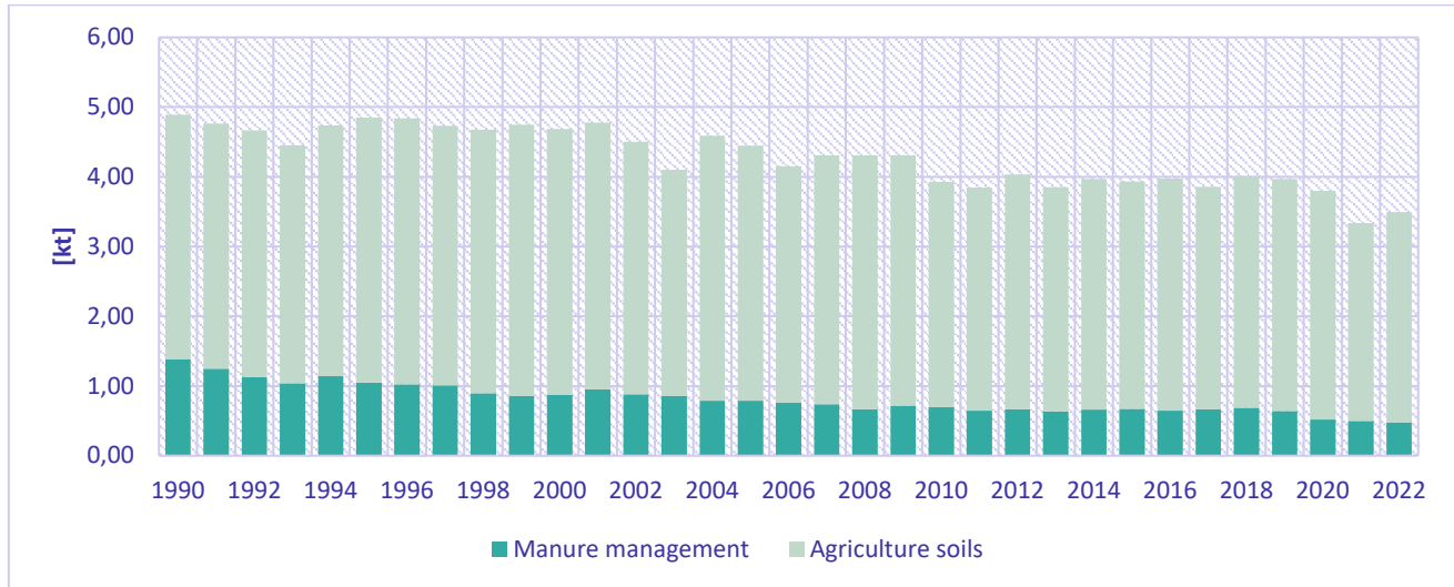
Figure 5.4: PM 10 emission trends by sectors
