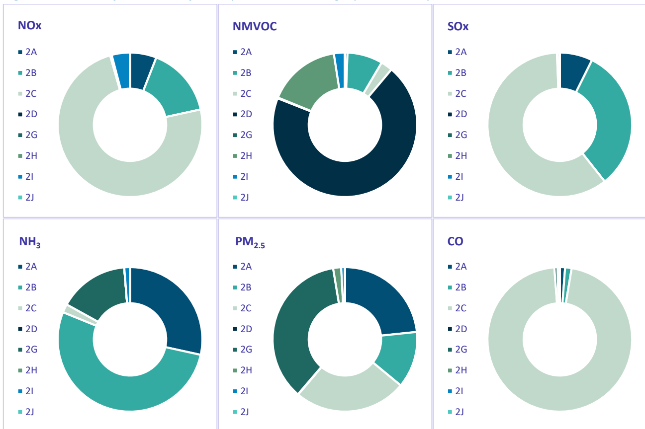
Figure 4.1: Share of emissions of main pollutants in category 2 – Industry in 2022
