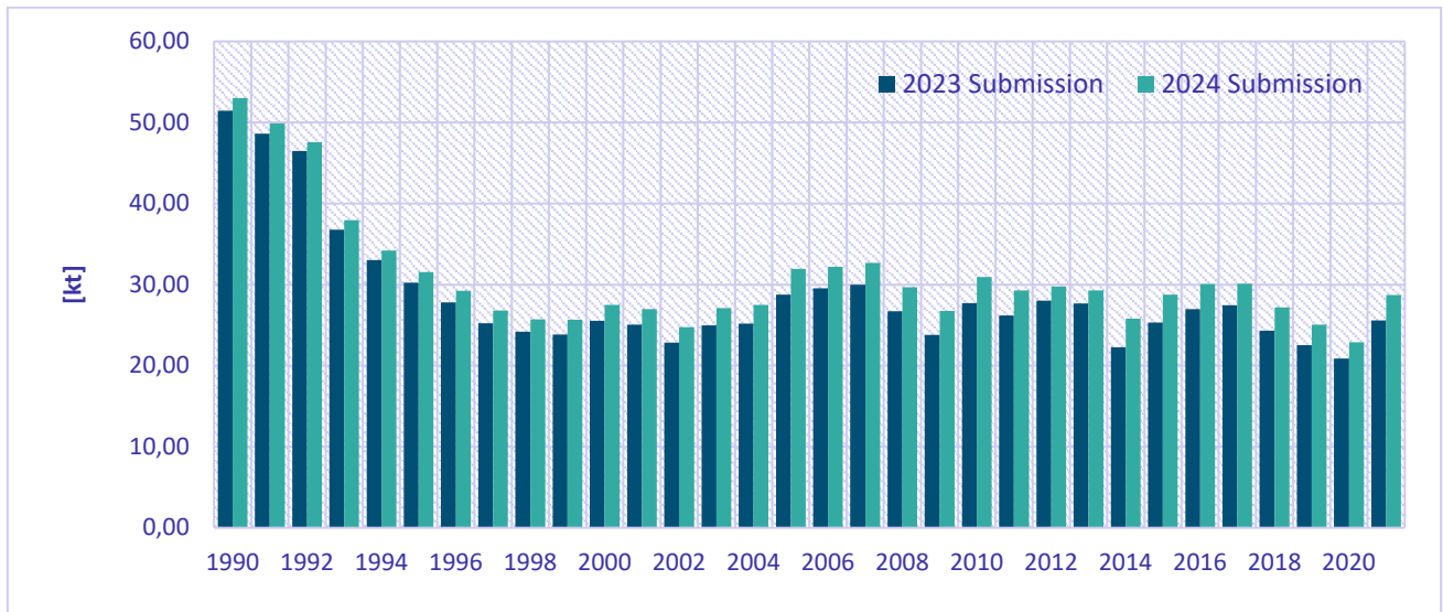
Figure 8.12: Comparison of PAHs emission total between the 2023 final submission and 2024 final submission
