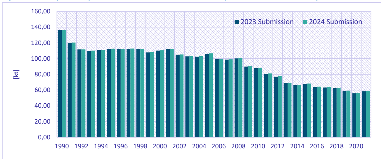
Figure 8.1: Comparison of NO x emission total between the 2023 final submission and 2024 final submission
