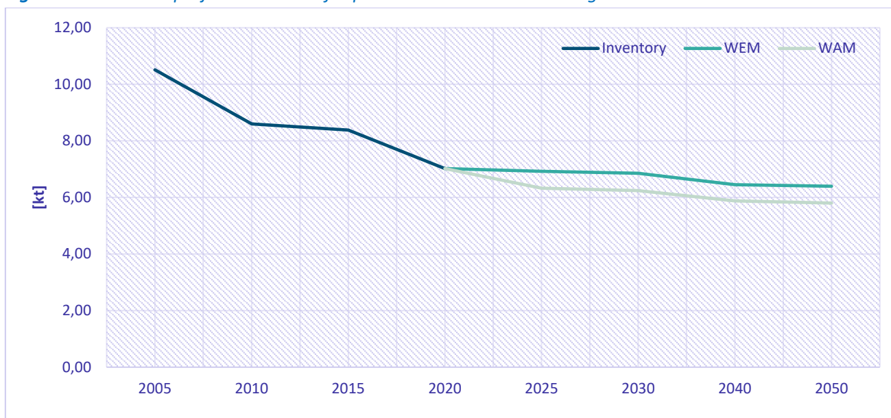
Figure 9.7: Emission projections trends for pollutant NMVOC in sector Agriculture
