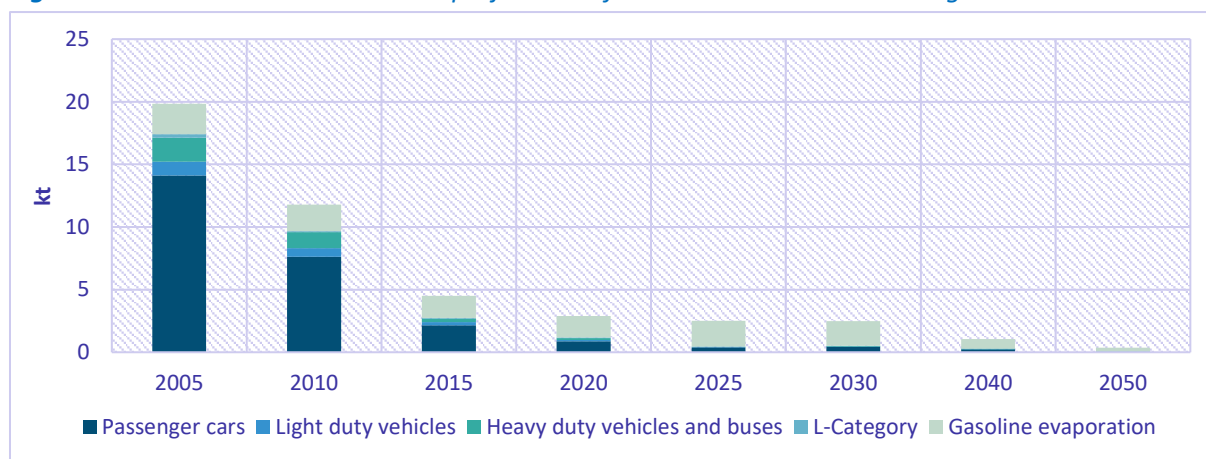
Figure 9.32: Historical emissions and projections of NMVOC emissions according to WAM scenario
