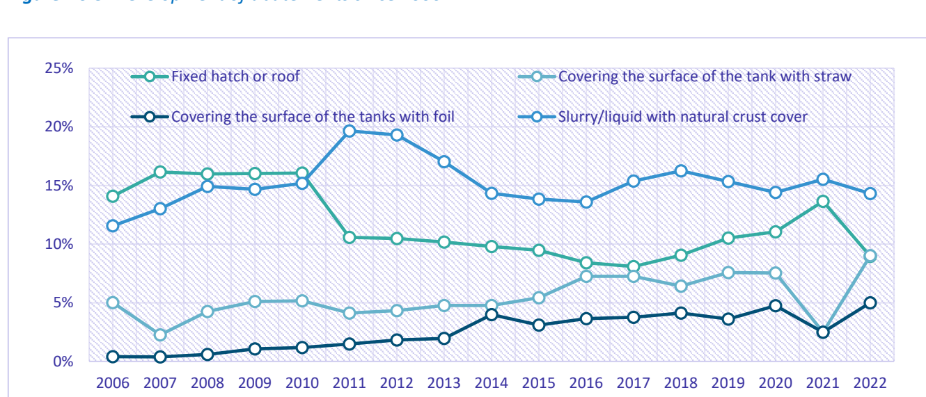
Figure A6.3: Development of abatements since 2006
