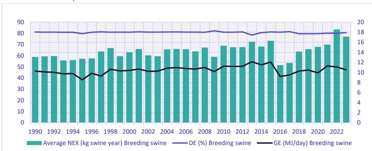
Figure 5.9: Trend of feed digestibility, nitrogen excretion rate and gross energy intake of breeding swine in the Slovak Republic in 1990-2023
