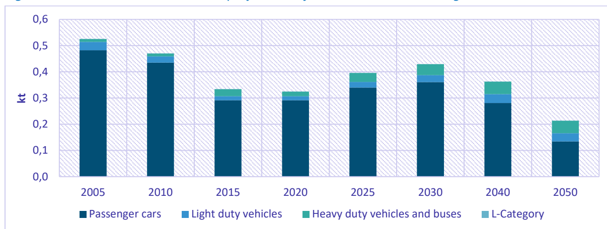
Figure 9.35: Historical emissions and projections of NH 3 emissions according to WEM scenario
