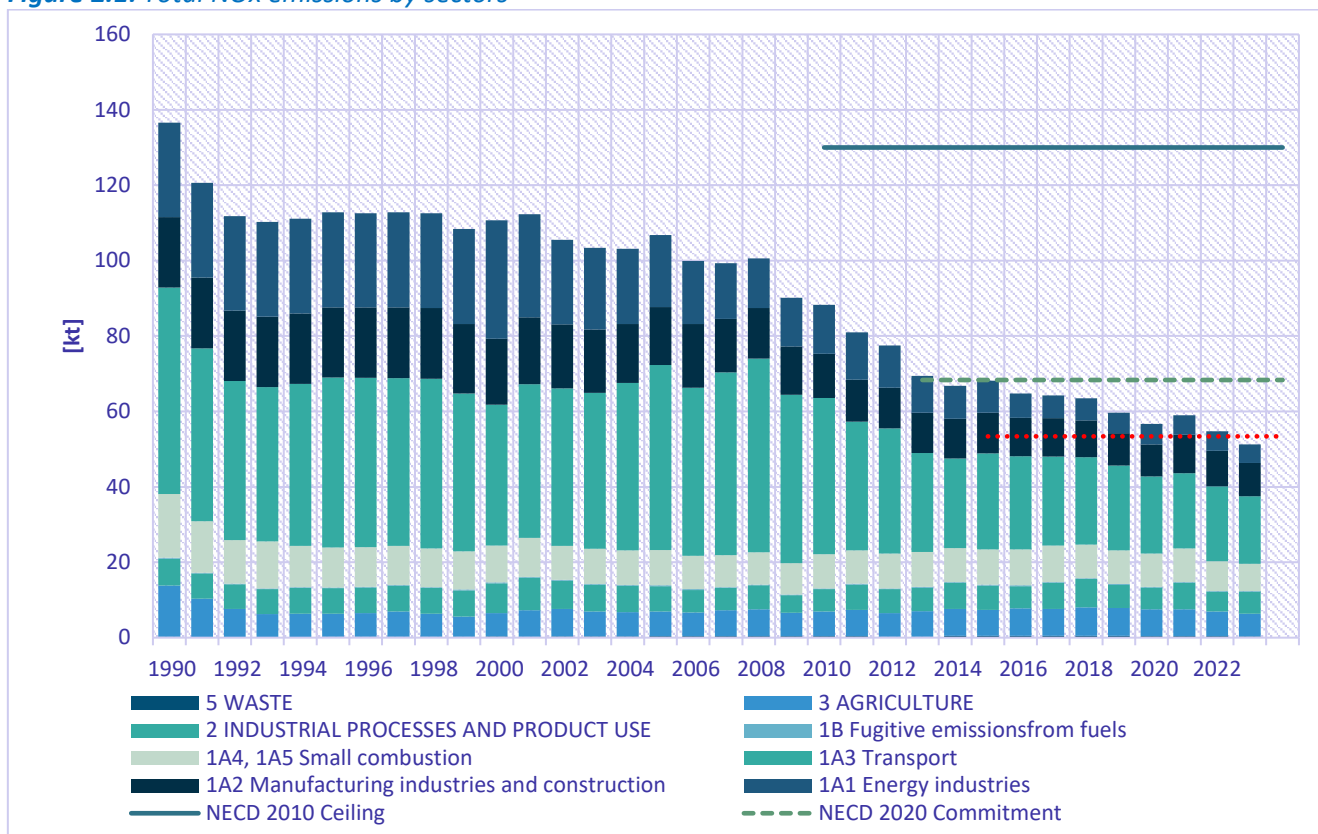
Figure 2.1: Total NO x emissions by sectors
