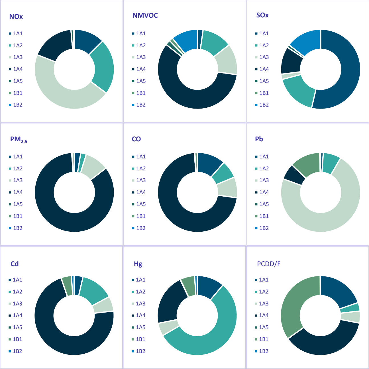
Figure 3.1: Shares of categories in emissions of individual pollutants in 2023 – energy sector
