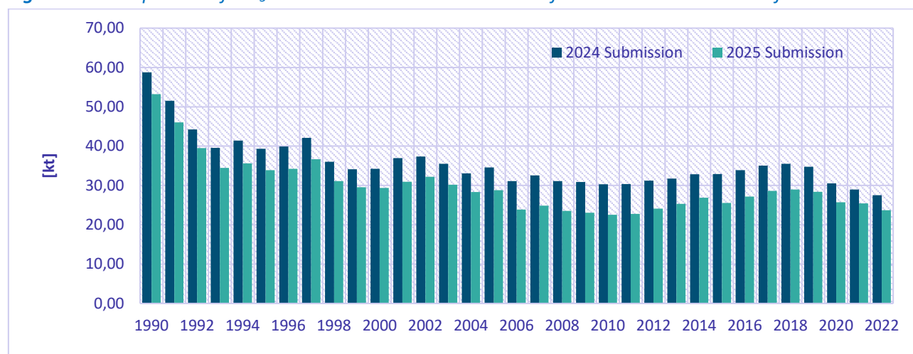
Figure 8.4: Comparison of NH 3 emission total between the 2024 final submission and 2025 final submission
