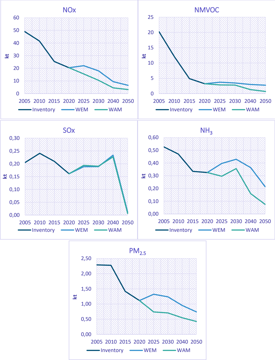
Figure 9.17: Air pollutants emissions trends in sector Transport
