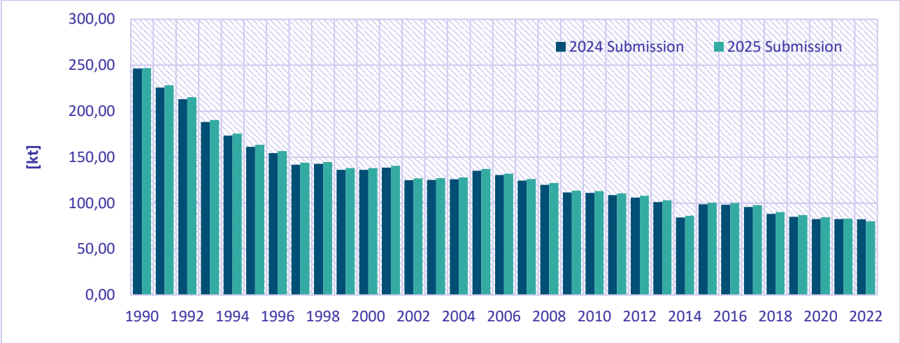
Figure 8.2: Comparison of NMVOC emission total between the 2024 final submission and 2025 final submission
