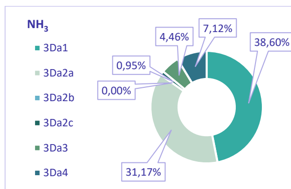
Figure 5.13: The share of NH 3 emissions by categories within agricultural soils in 2023
