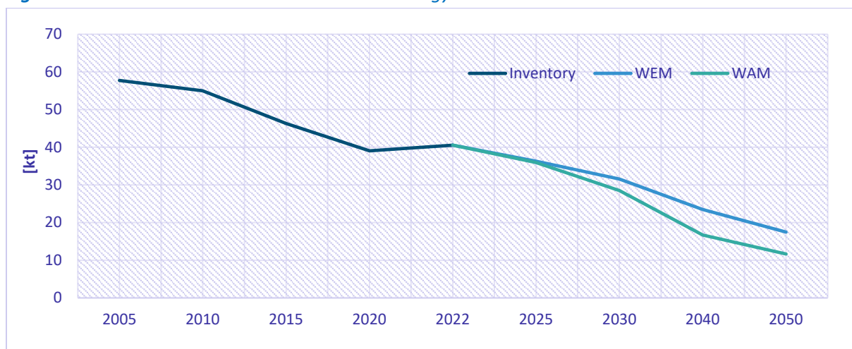
Figure 9.8: NMVOC emissions trends in sector Energy
