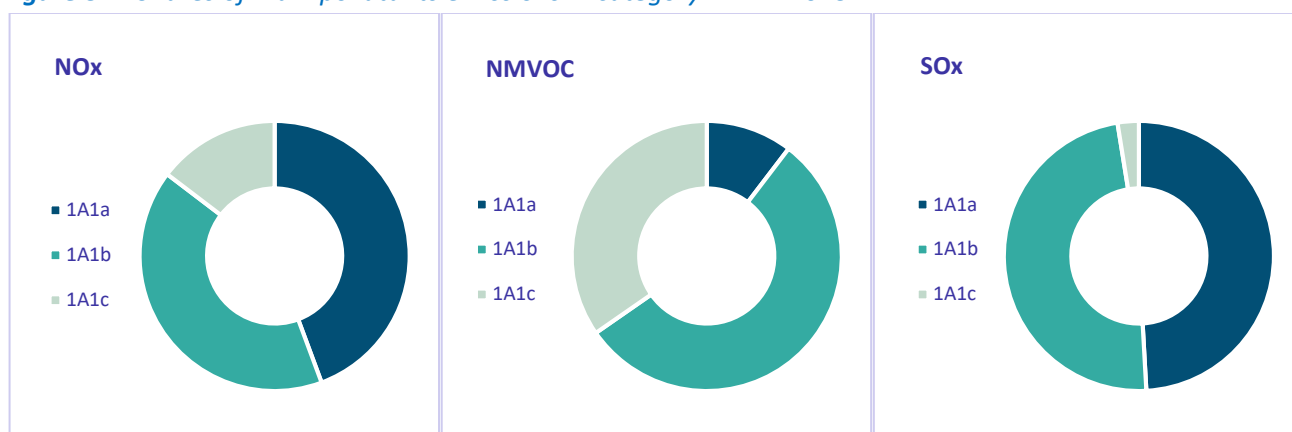
Figure 3.2: Shares of main pollutants emissions in category 1A1 in 2023
