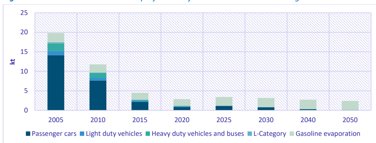
Figure 9.31: Historical emissions and projections of NMVOC emissions according to WEM scenario
