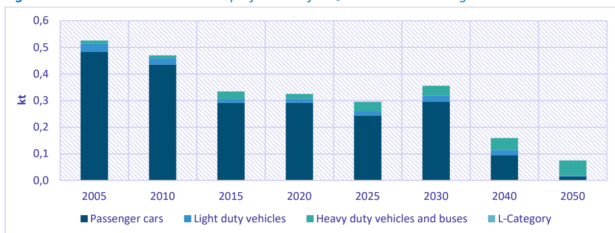
Figure 9.36: Historical emissions and projections of NH 3 emissions according to WAM scenario
