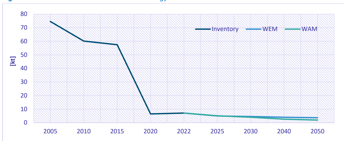
Figure 9.9: SOx emissions trends in sector Energy
