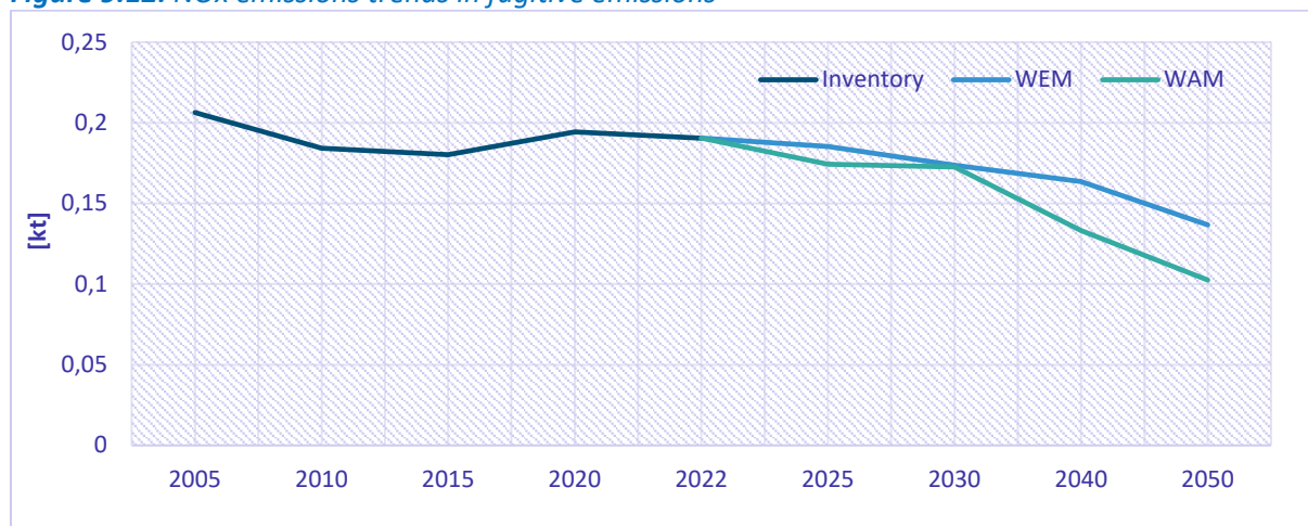
Figure 9.12: NO x emissions trends in fugitive emissions
