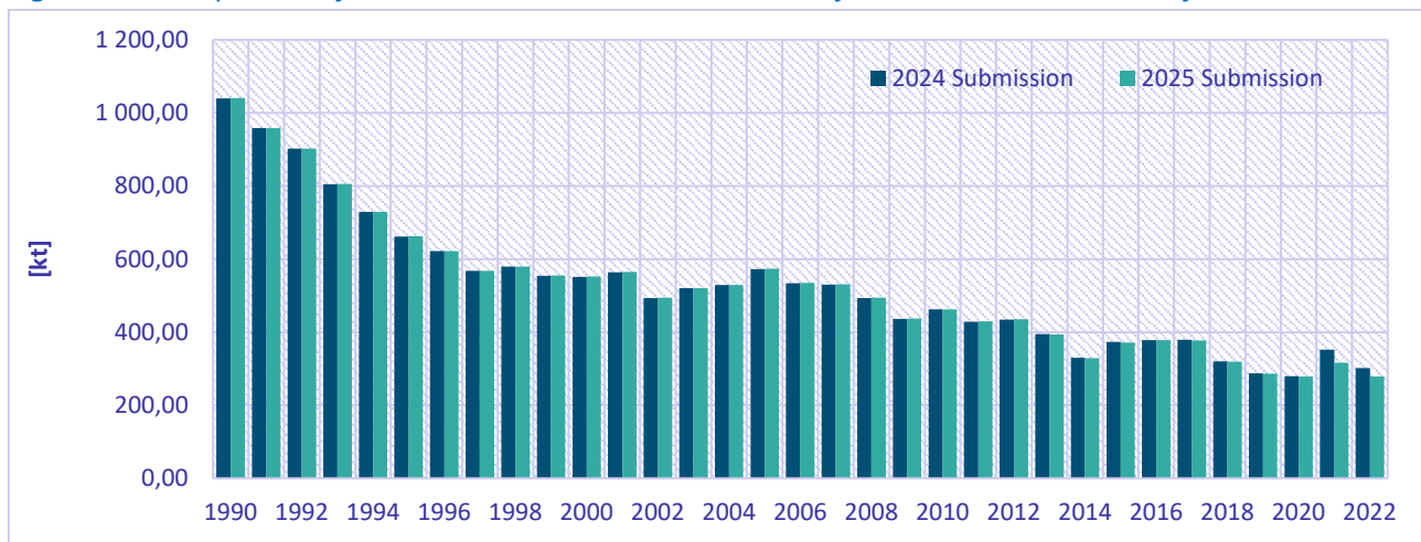
Figure 8.7: Comparison of CO emission total between the 2024 final submission and 2025 final submission
