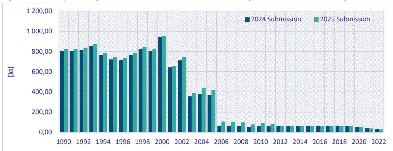
Figure 8.11: Comparison of PCDD/F emission total between the 2024 final submission and 2025 final submission
