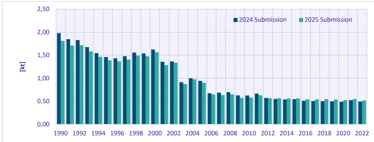
Figure 8.10: Comparison of Hg emission total between the 2024 final submission and 2025 final submission
