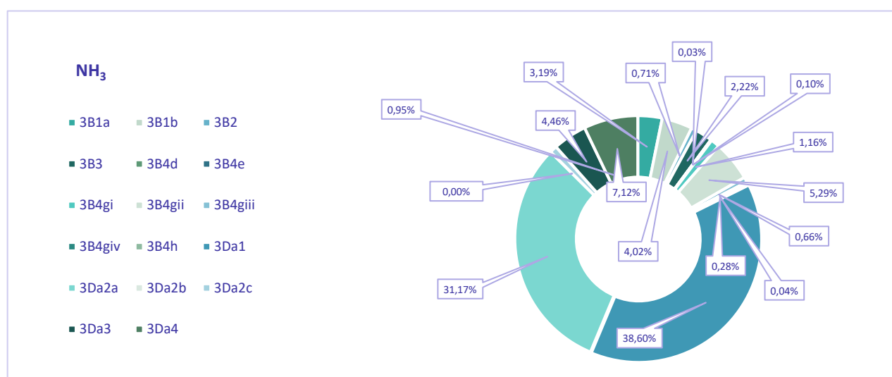
Figure 5.2: NH 3 emissions per subsectors in %
