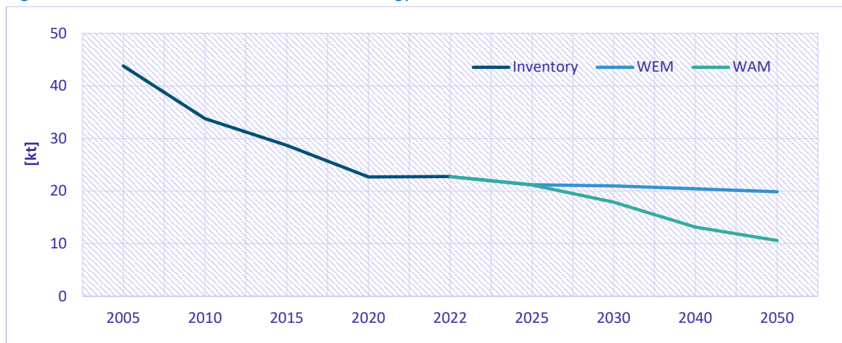
Figure 9.7: NOx emissions trends in sector Energy
