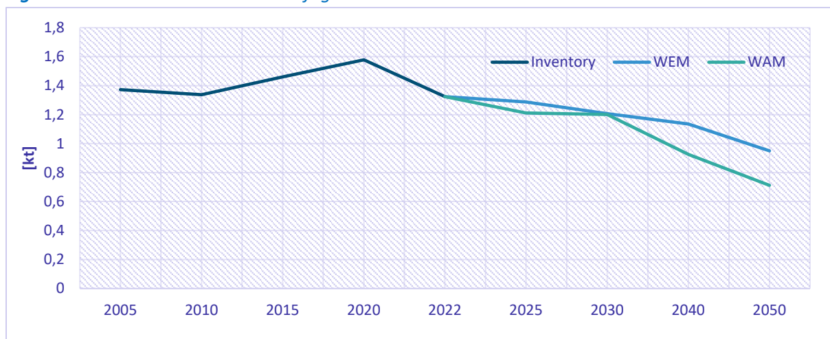
Figure 9.14: SO x emissions trends in fugitive emissions
