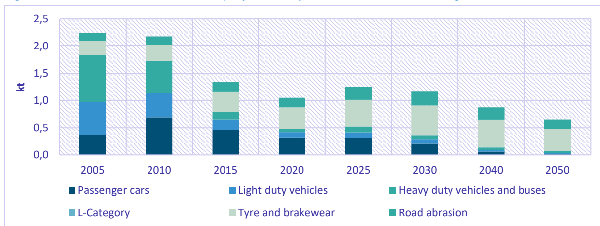
Figure 9.30: Historical emissions and projections of PM 2.5 emissions according to WAM scenario
