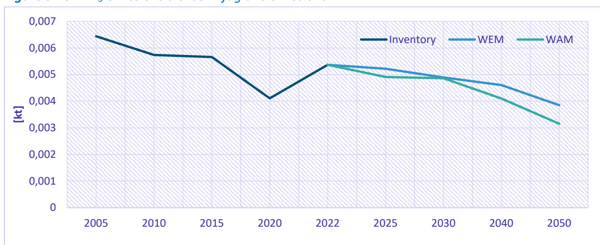
Figure 9.15: NH 3 emissions trends in fugitive emissions
