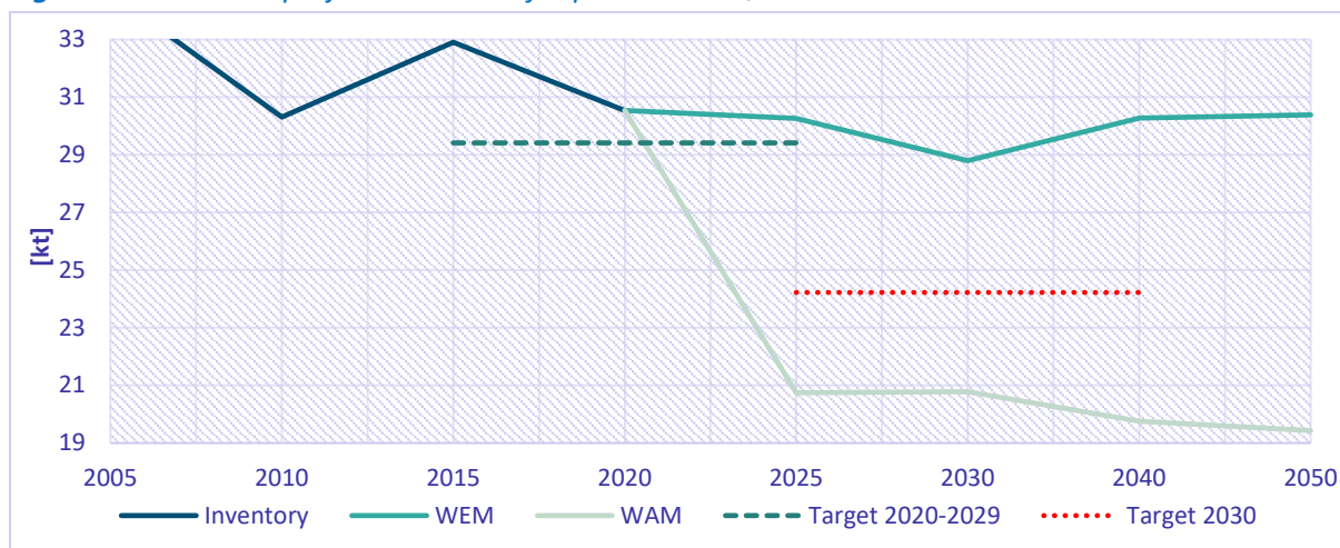
Figure 9.4: Emission projections trends for pollutant NH 3
