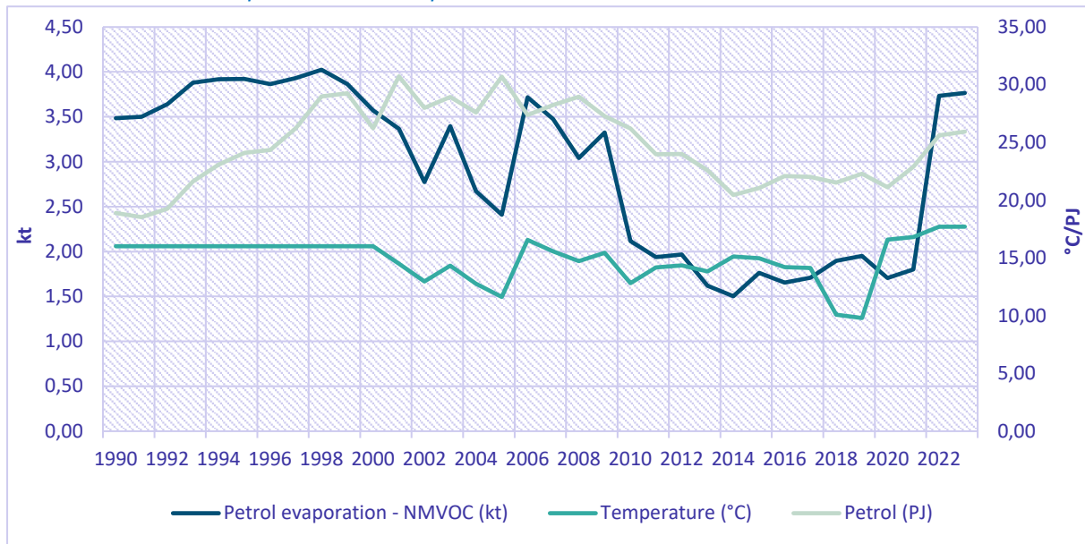
Figure 3.8: Ambient air temperature and evaporation emissions correlation
