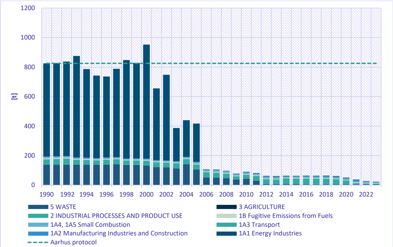
Figure 2.12: Total PCDD/PCDF emissions by sectors
