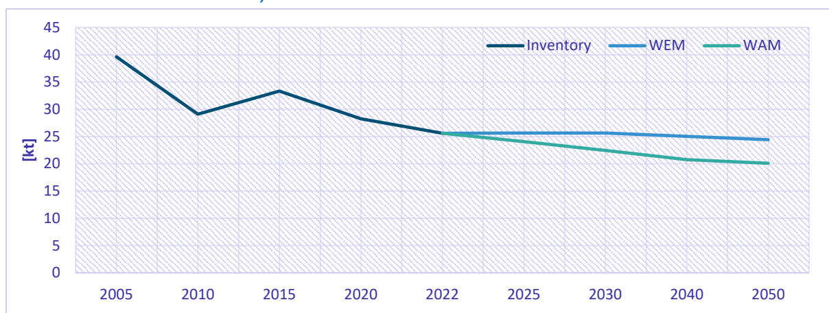
Figure 9.38: Historical emissions and projections of NMVOC emissions according to WEM and WAM scenario in Industry sector
