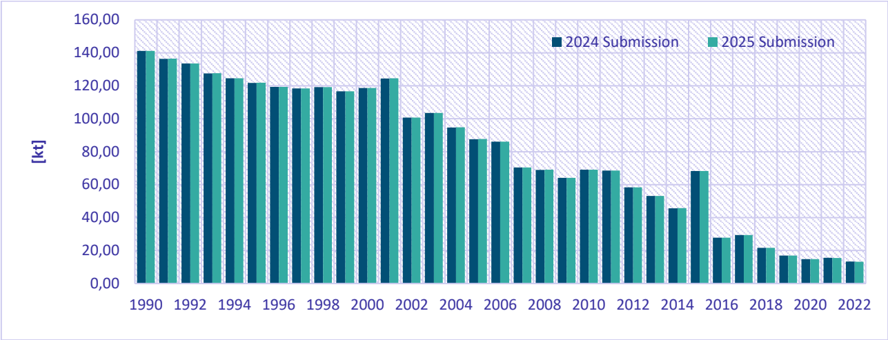
Figure 8.3: Comparison of SOx emission total between the 2024 final submission and 2025 final submission
