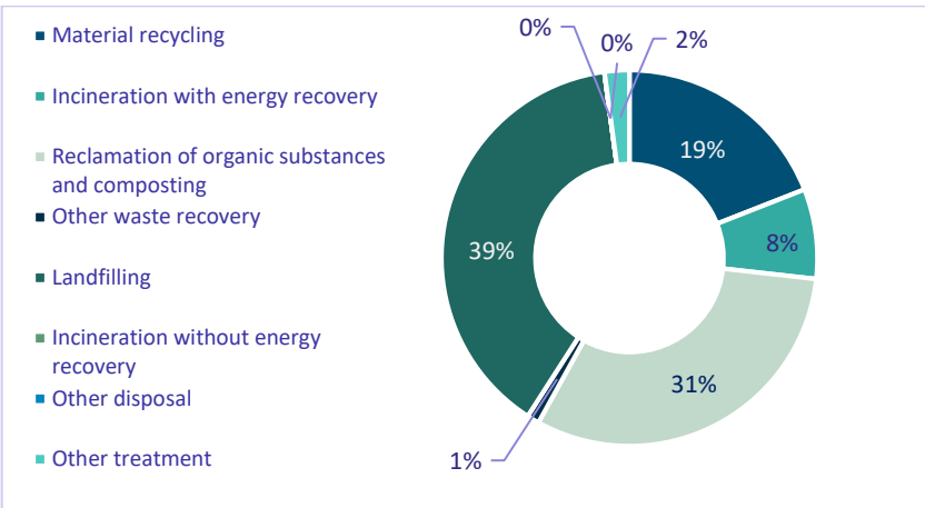
Figure 6.1: Municipal waste treatment in the Slovak Republic in 2023
