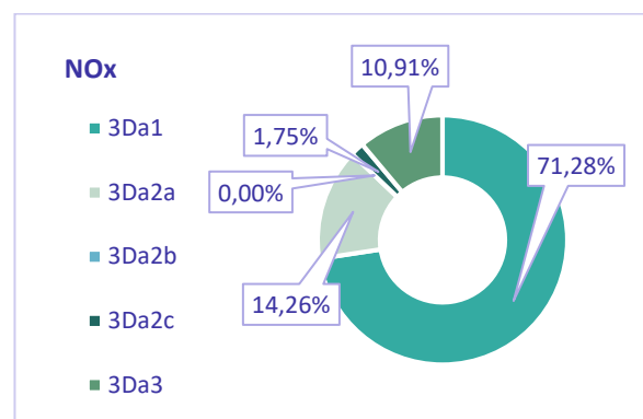
Figure 5.14: The share of NO x emissions by categories within agricultural soils in 2023
