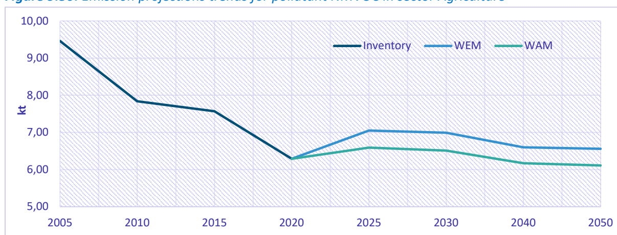
Figure 9.50: Emission projections trends for pollutant NMVOC in sector Agriculture
