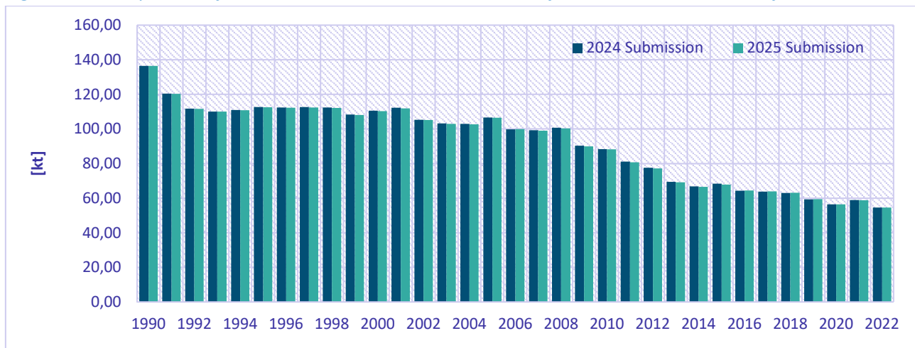
Figure 8.1: Comparison of NO x emission total between the 2024 final submission and 2025 final submission
