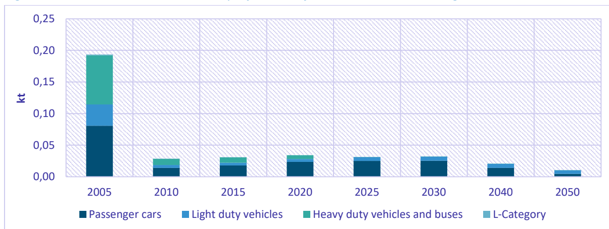
Figure 9.34: Historical emissions and projections of SOx emissions according to WAM scenario
