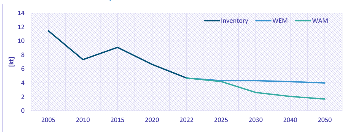
Figure 9.39: Historical emissions and projections of SO x emissions according to WEM and WAM scenario in Industry sector
