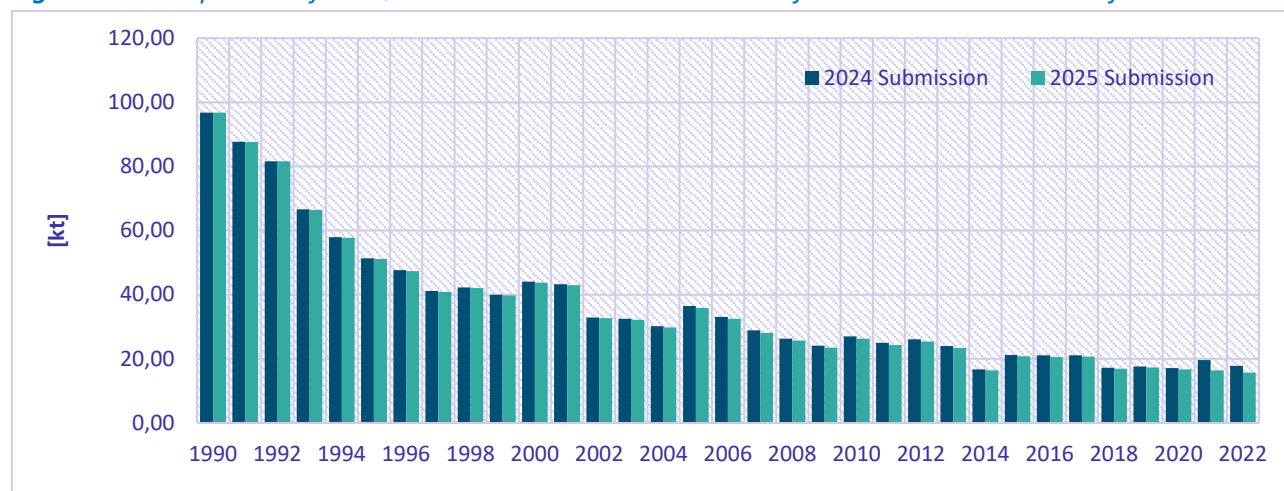
Figure 8.5: Comparison of PM 2.5 emission total between the 2024 final submission and 2025 final submission
