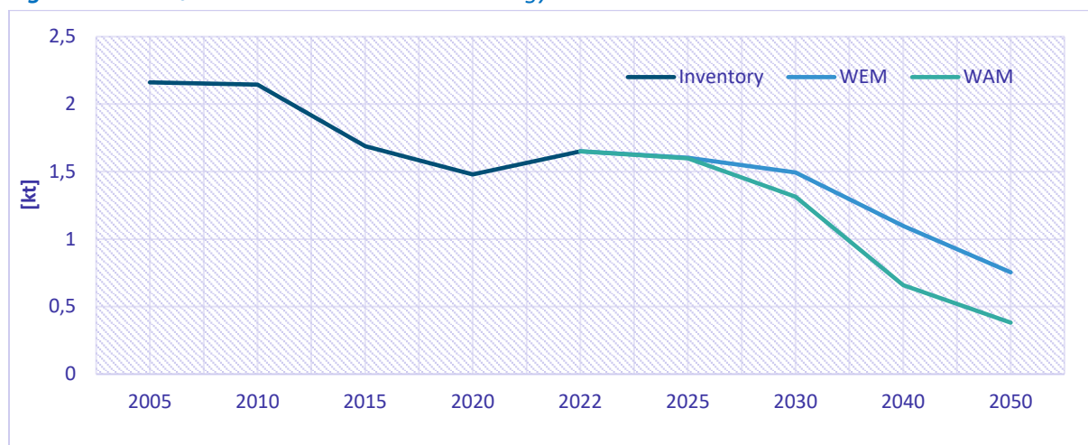
Figure 9.11: PM_{2.5} emissions trends in sector Energy
