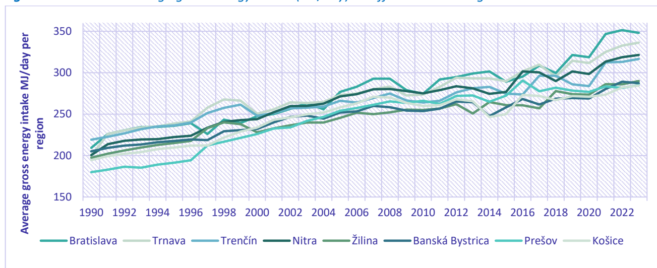
Figure 5.6: Trend in average gross energy intake (MJ/day) in different Slovak regions
