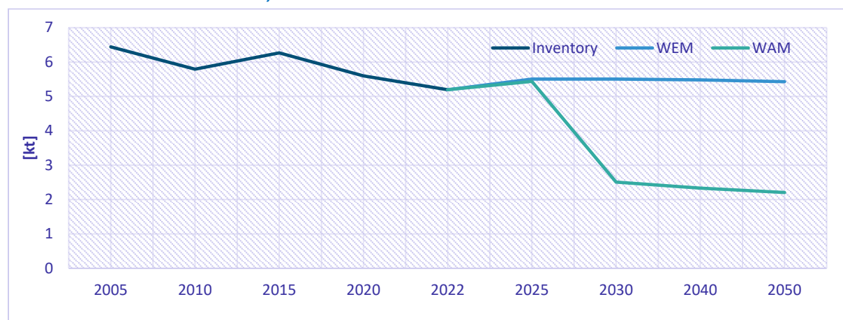
Figure 9.37: Historical emissions and projections of NO x emissions according to WEM and WAM scenario in Industry sector
