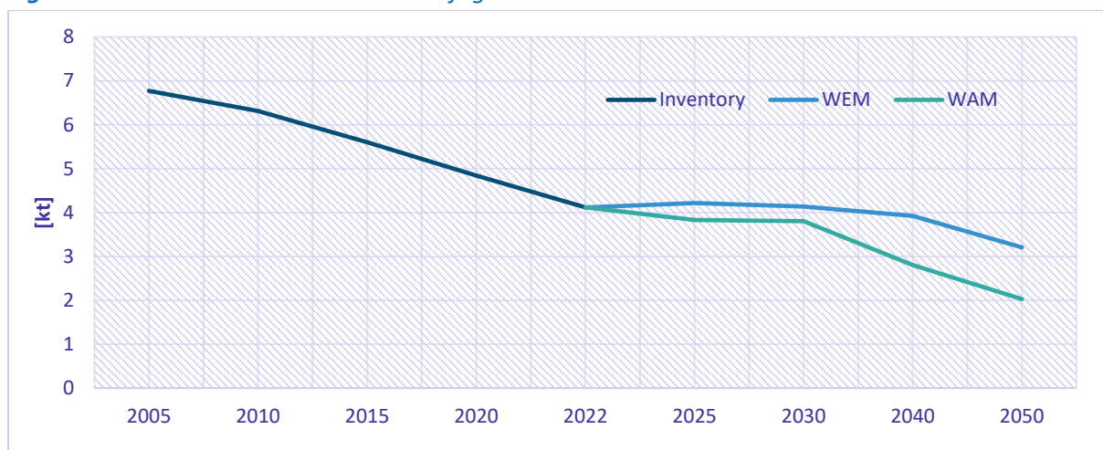
Figure 9.13: NMVOC emissions trends in fugitive emissions
