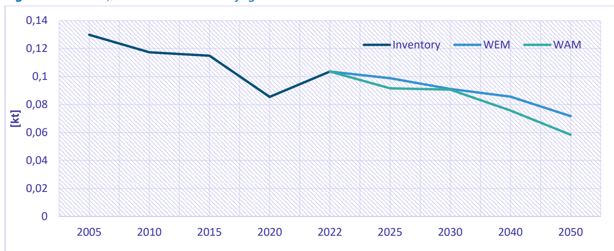
Figure 9.16: PM 2.5 emissions trends in fugitive emissions
