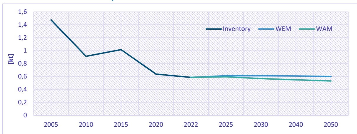
Figure 9.41: Historical emissions and projections of PM 2.5 emissions according to WEM and WAM scenario in Industry sector
