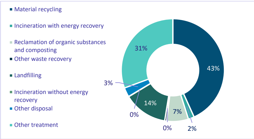
Figure 6.2: Industrial waste treatment in the Slovak Republic in 2023
