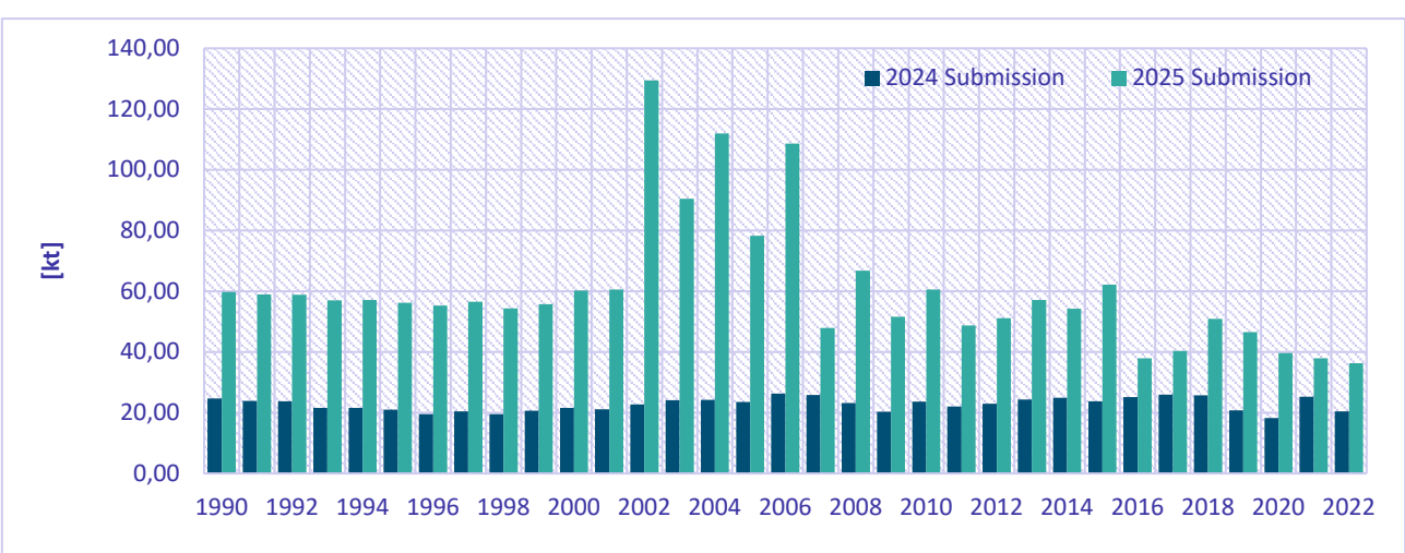
Figure 8.14: Comparison of PCBs emission total between the 2024 final submission and 2025 final submission
