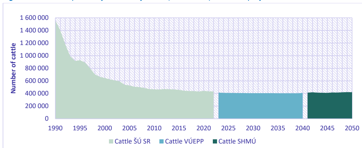
Figure 9.42: Development of number of cattle (1990-2023) and their projections until 2050
