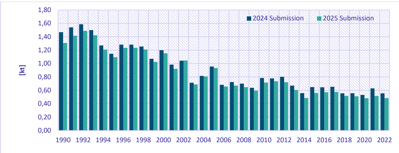
Figure 8.9: Comparison of Cd emission total between the 2024 final submission and 2025 final submission
