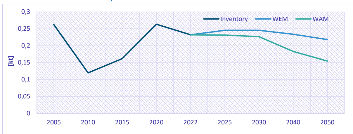
Figure 9.40: Historical emissions and projections of NH 3 emissions according to WEM and WAM scenario in Industry sector
