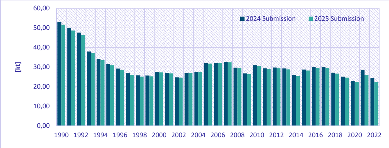
Figure 8.12: Comparison of PAHs emission total between the 2024 final submission and 2025 final submission
