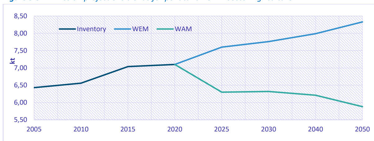
Figure 9.52: Emission projections trends for pollutant NO x in sector Agriculture
