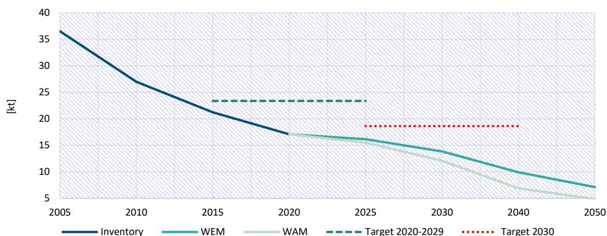
Figure 8.2.5: Emission projections trends for pollutant \text{PM}_{2.5}
